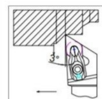
DDJNR/L Series
