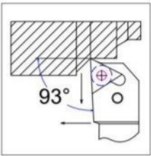
PTJNR/L Series
