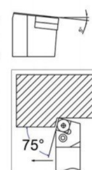
PSBNR/L-A Series
