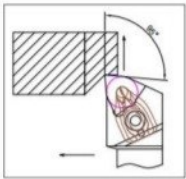
DWLNR/L Series
