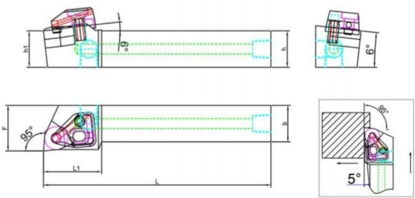
DWLNR/L-A Series
