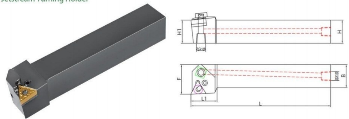
Jetstream Turning Holder
